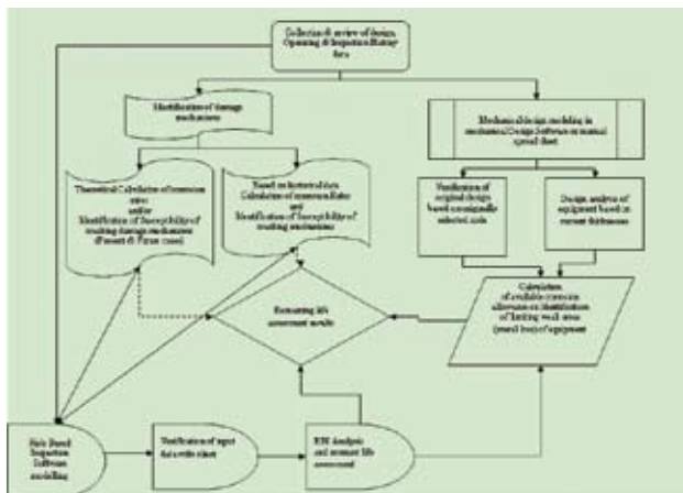
Concept for Remnant life Assessment
