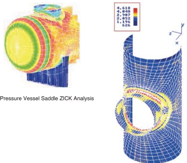
Nozzle FE Analysis against Load
